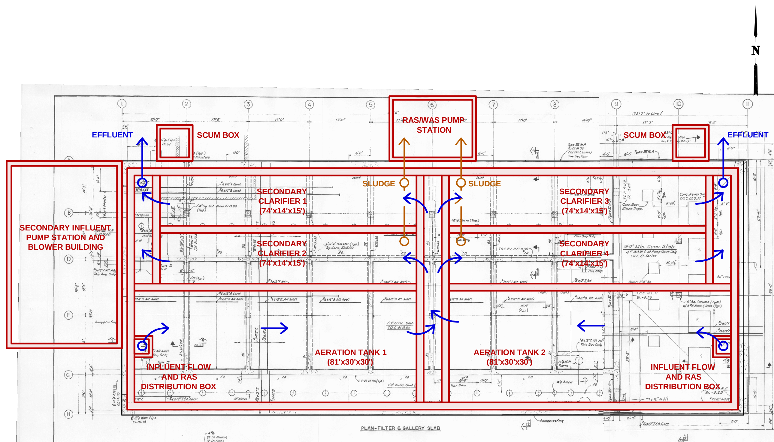
WWMP PILOTING - PHASE 1 ENGINEERING EVALUATION PEIRCE ISLAND WWTF - PORTSMOUTH, NH CAS WITH BIOMAG CONVENTIONAL SECONDARY TREATMENT
