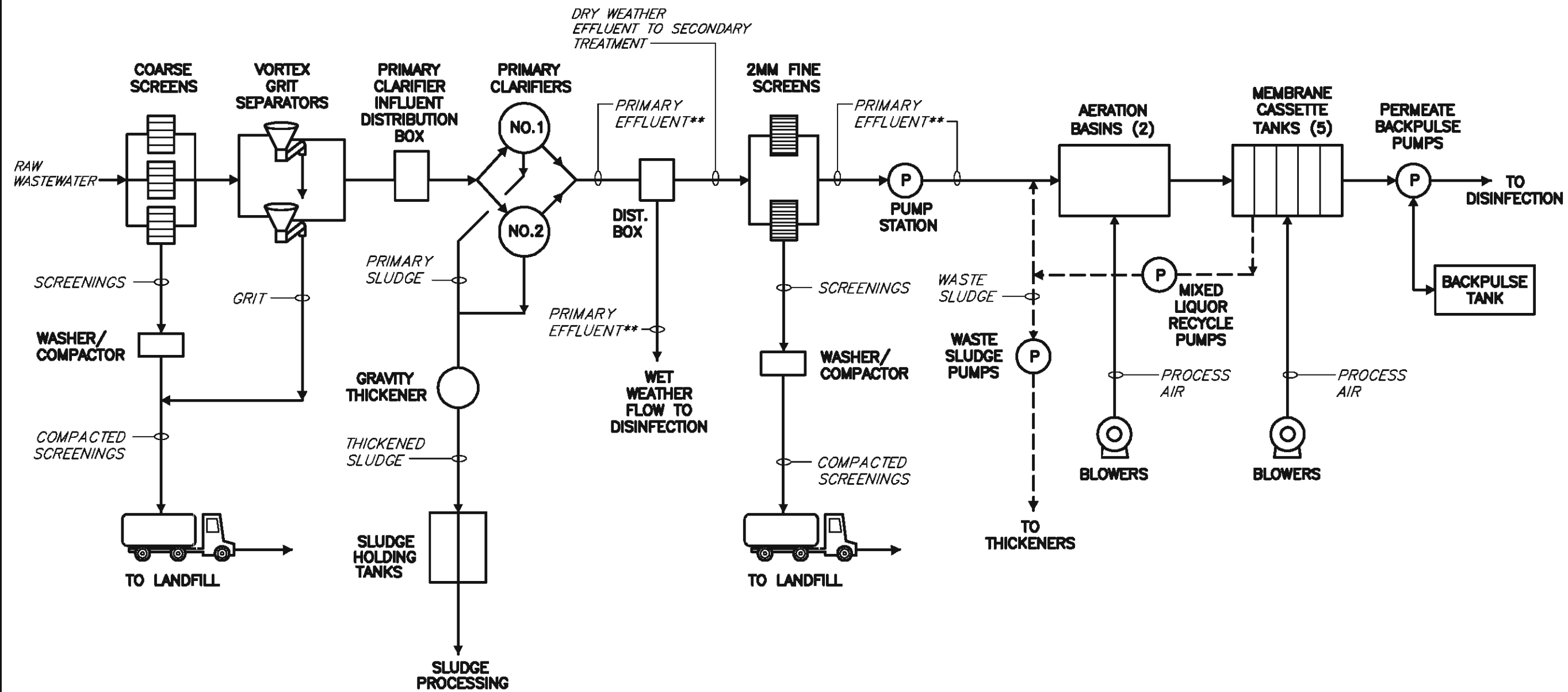
OPTION 7 FIG. 7-CST-PFS PROCESS FLOW SCHEMATIC WWMP PILOTING - PHASE 1 ENGINEERING EVALUATION PEIRCE ISLAND WWTF - PORTSMOUTH, NH MBR CONVENTIONAL SECONDARY TREATMENT
