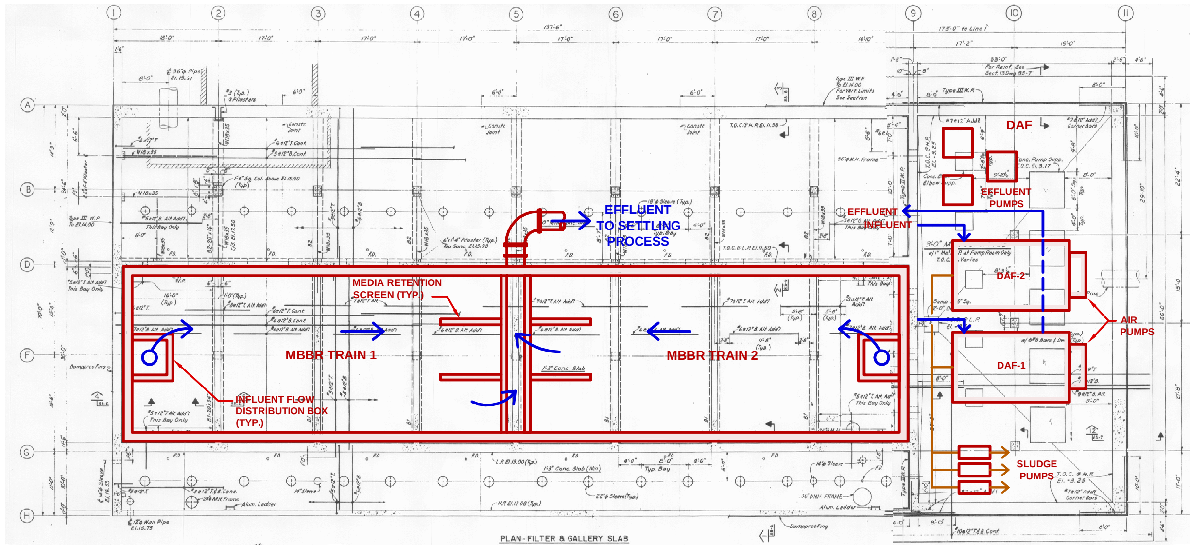
PLAN-FILTER & GALLERY SLAB
