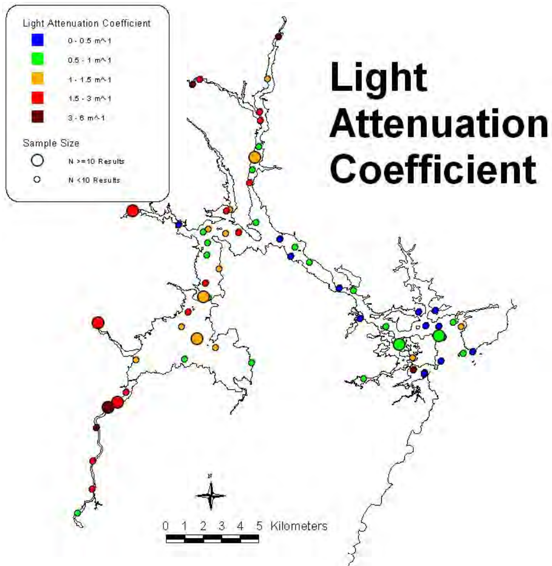
Figure 32: Median Light Attenuation Coefficient at Water Quality Stations
