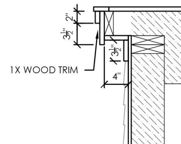
8 RAKE 3/4" = 1'-0"
