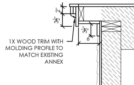
7 RAKE 3/4" = 1'-0"
