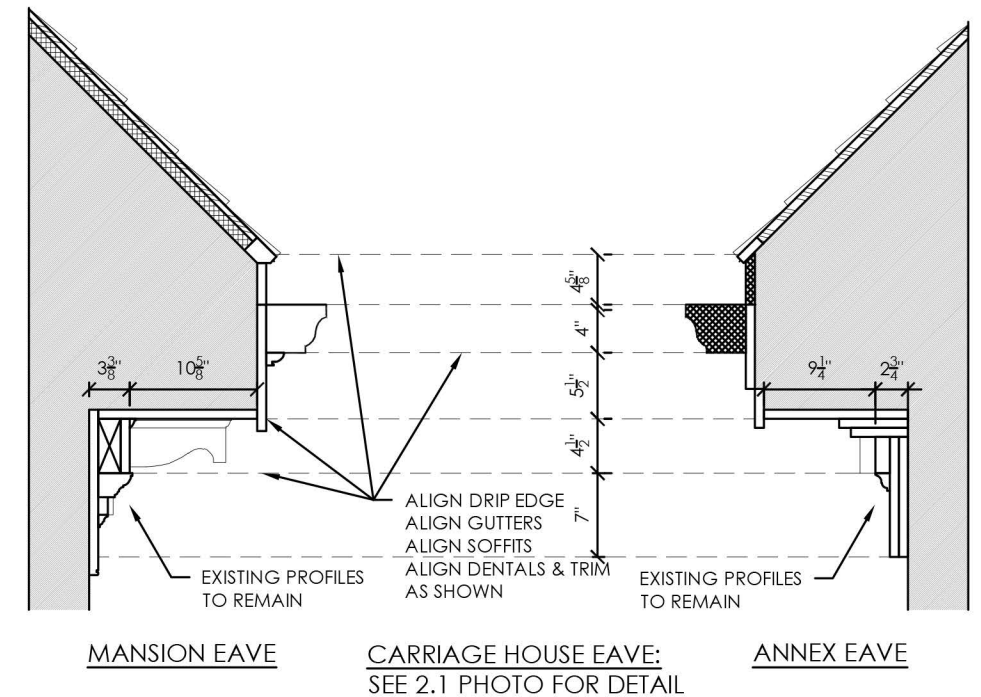
9 EAVE REFERENCE 3/4" = 1'-0"
