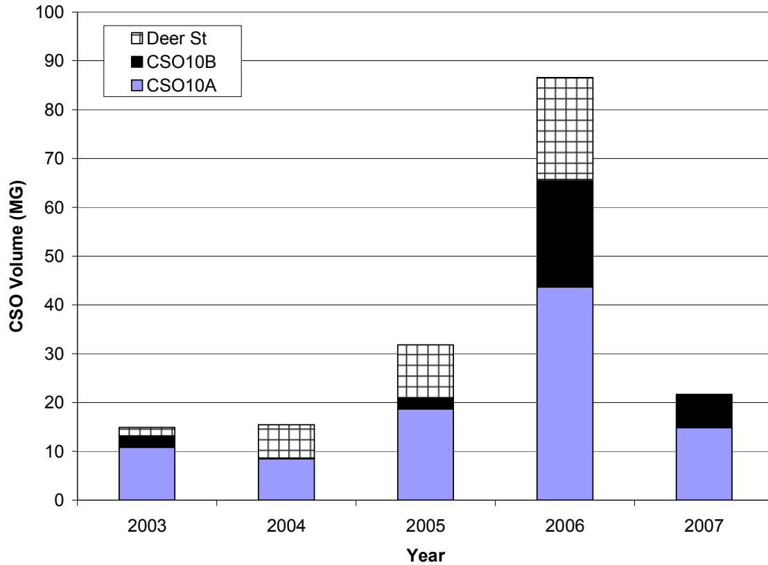
Figure 3.8 Annual CSO Volumes 2003-2007 (1)
