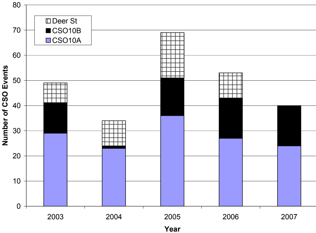
Figure 3.7 Annual CSO Activations 2003-2007 (1)
