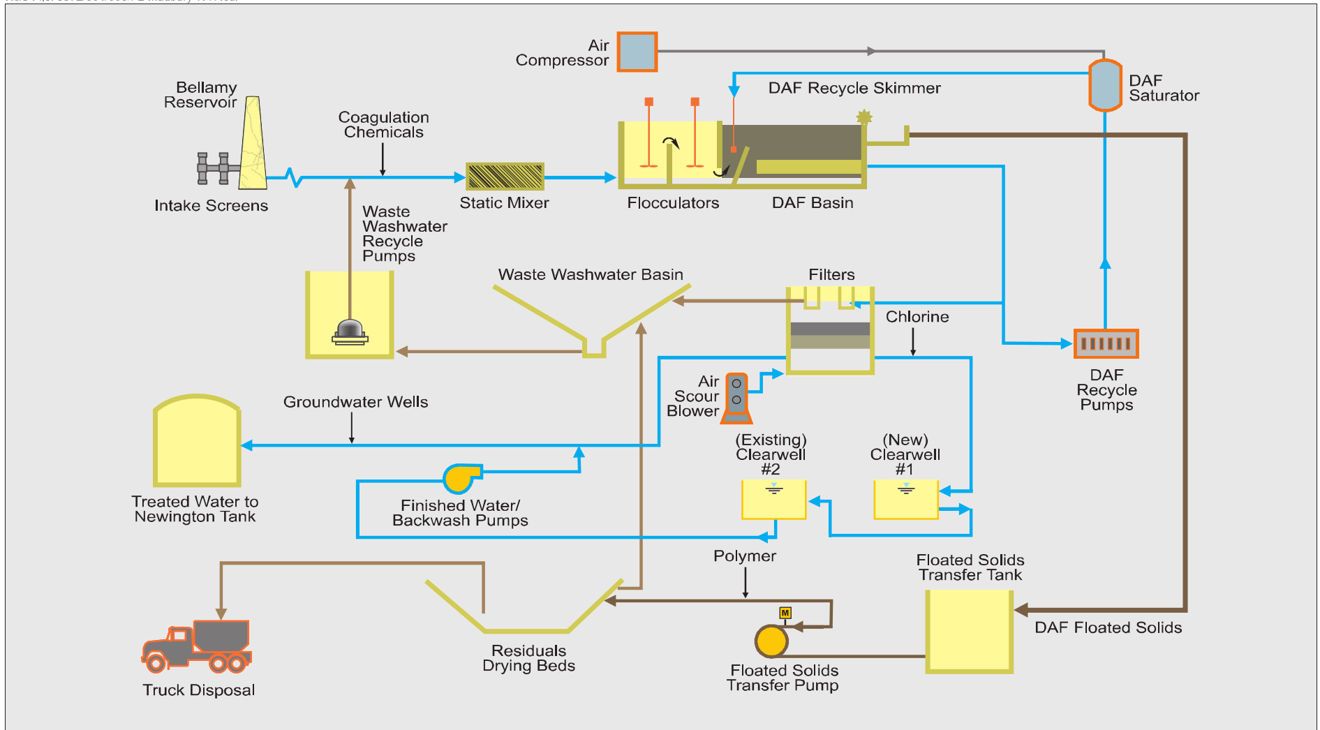
Madbury WTP Process Flow Diagram
