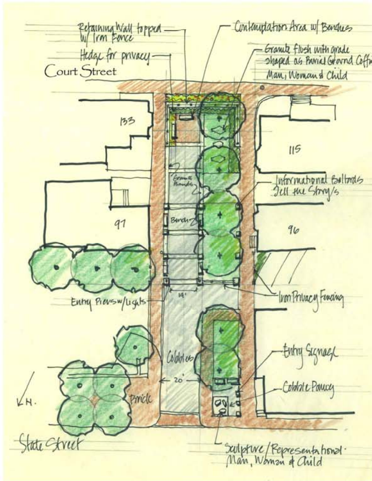
Information Bollard
